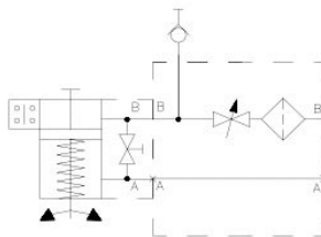
Block for Single Acting CBI-S-H
